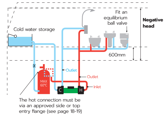
Figure 8: Negative head
