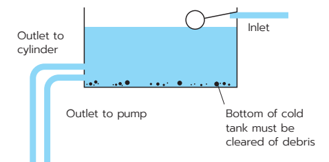
Figure 1: Tank inlet and outlet position
