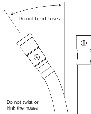
Figure 5: Couplers
