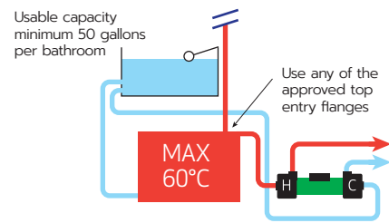
Figure 21: Horizontal cylinders
