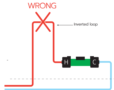
Figure 24: Inverted loops
