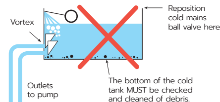
Figure 15: Aeration
