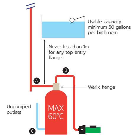
Figure 23: Warix flange
